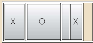
Available in 2-lite and 3-lite sliders. "X" designates operating lites and "O" designates fixed lites.
